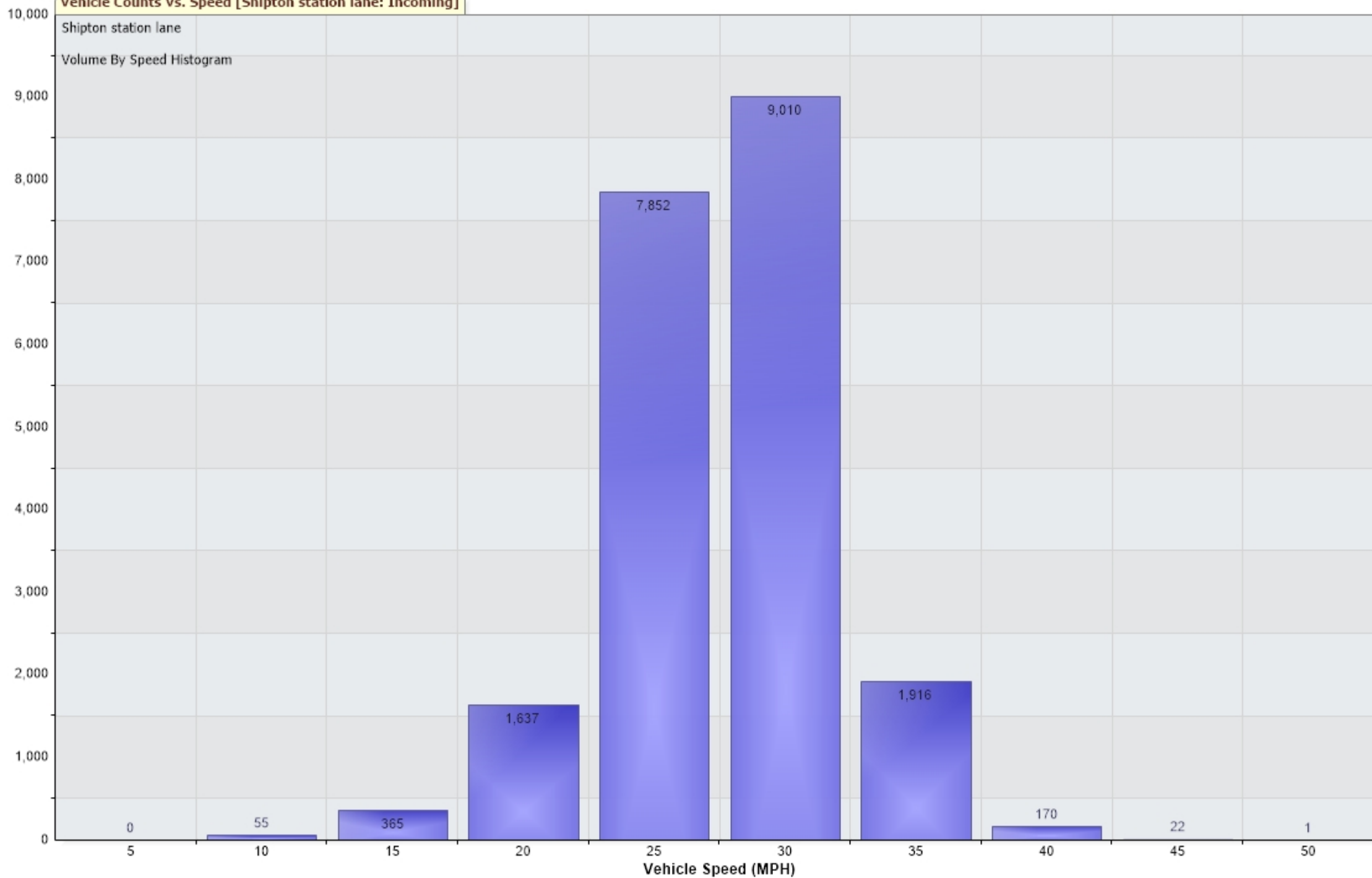
Vehicle Counts Vs. Speed [Shipton station lane: Incoming]
