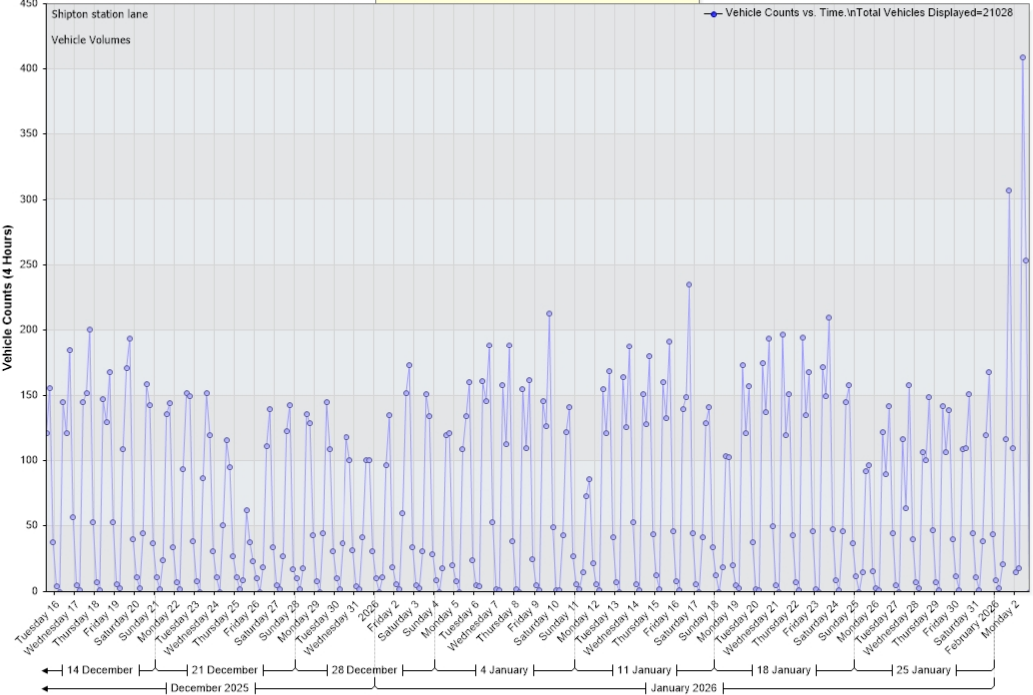
Vehicle Counts vs. Time [Shipton station lane: Incoming]
