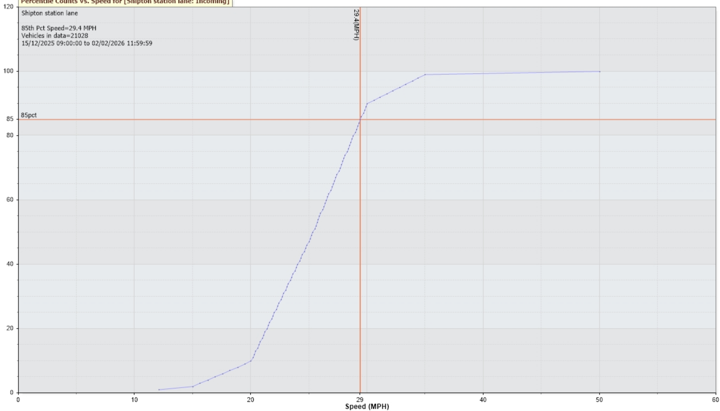
Percentile Counts Vs. Speed for [Shipton station lane: Incoming]
