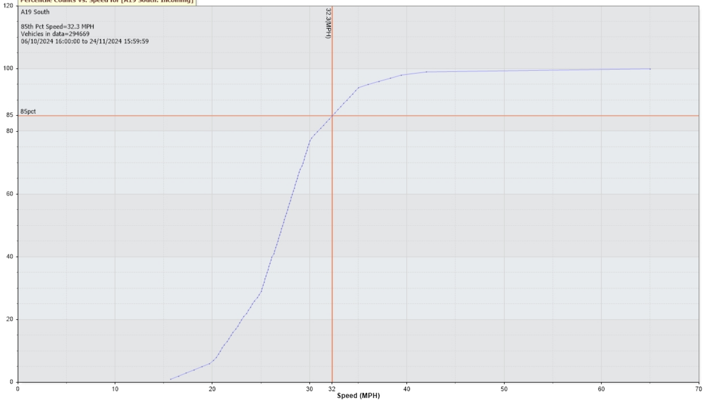
Percentile Counts Vs. Speed for [A19 South: Incoming]
