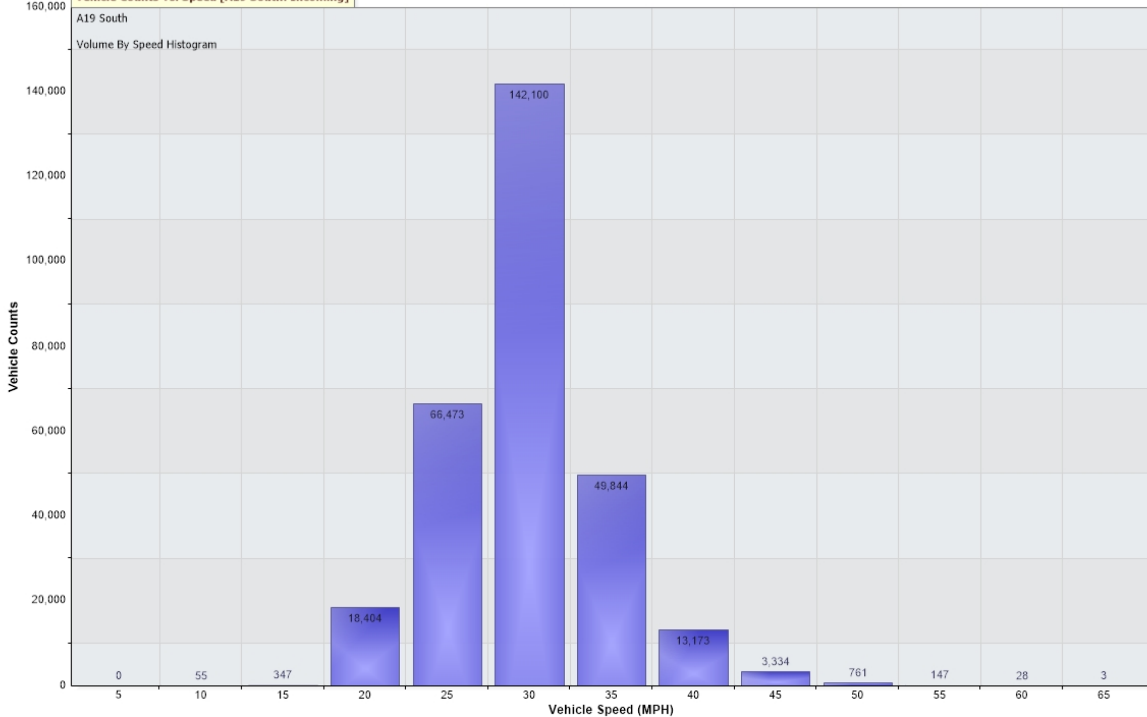
Vehicle Counts Vs. Speed [A19 South: Incoming]
