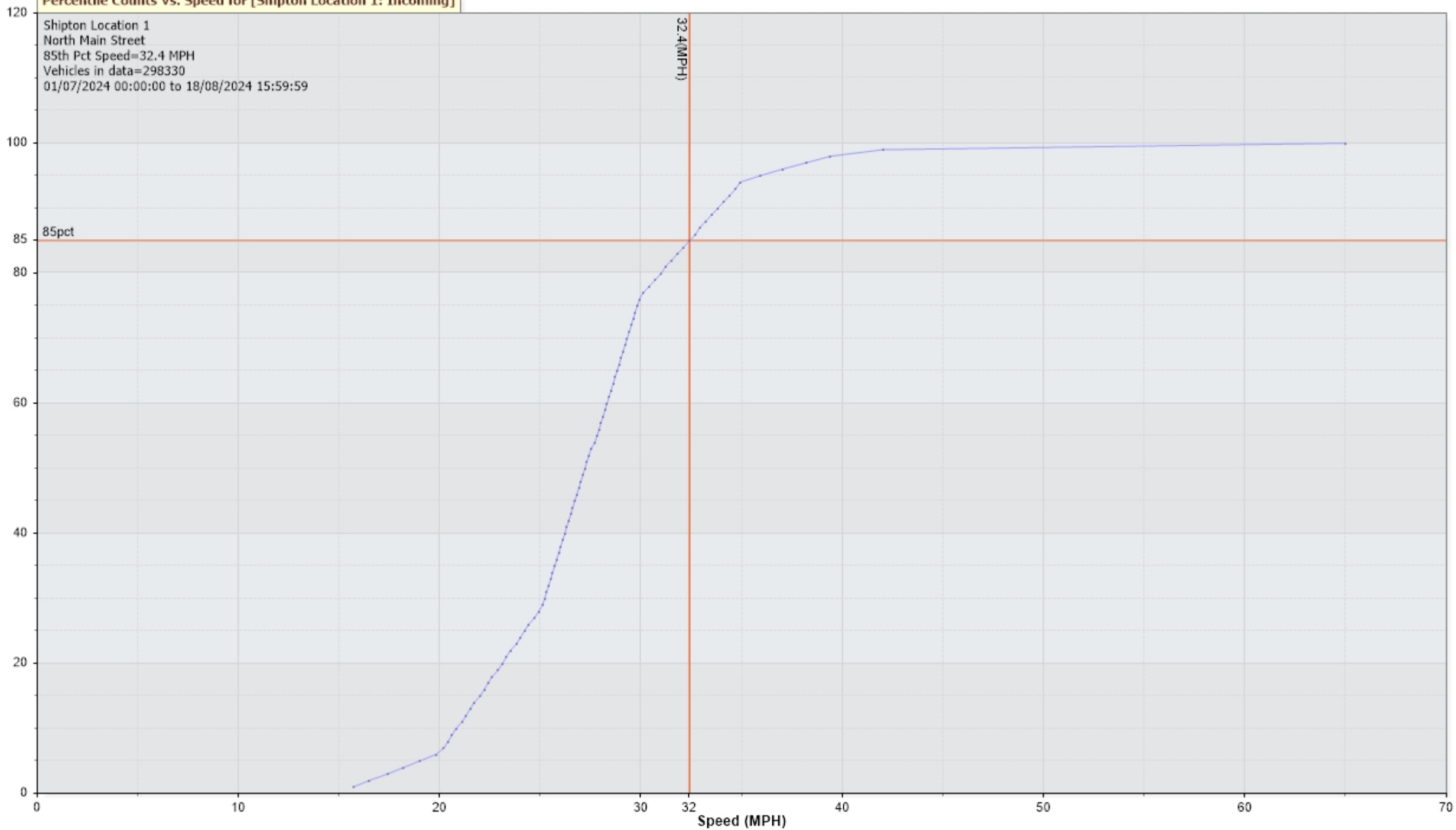
Percentile Counts Vs. Speed for [Shipton Location 1: Incoming]
