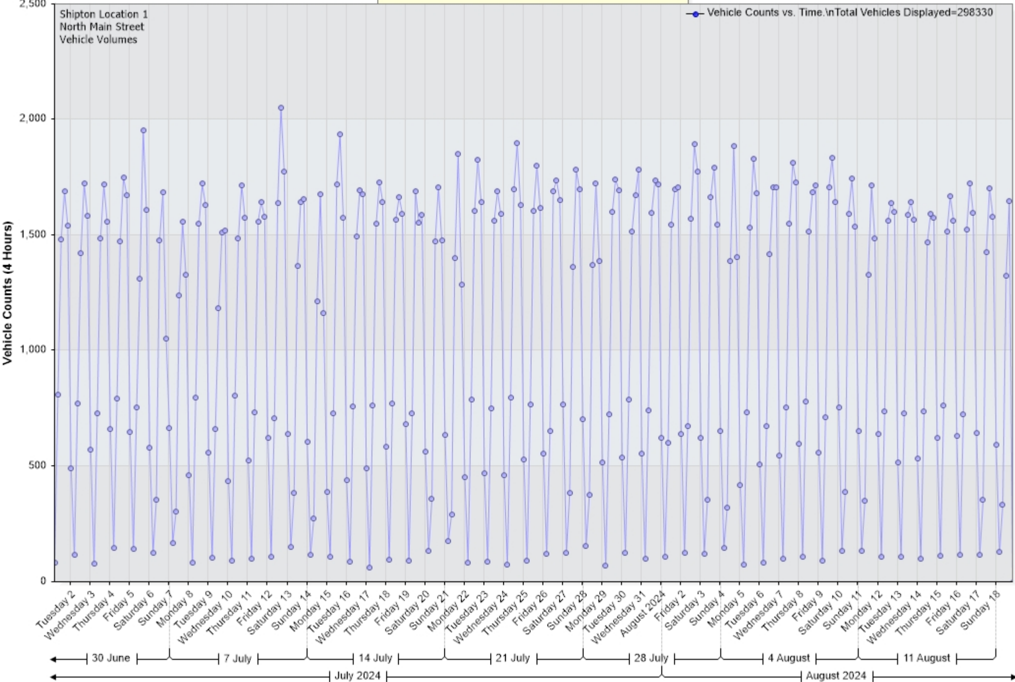
Vehicle Counts vs. Time [Shipton Location 1: Incoming]
