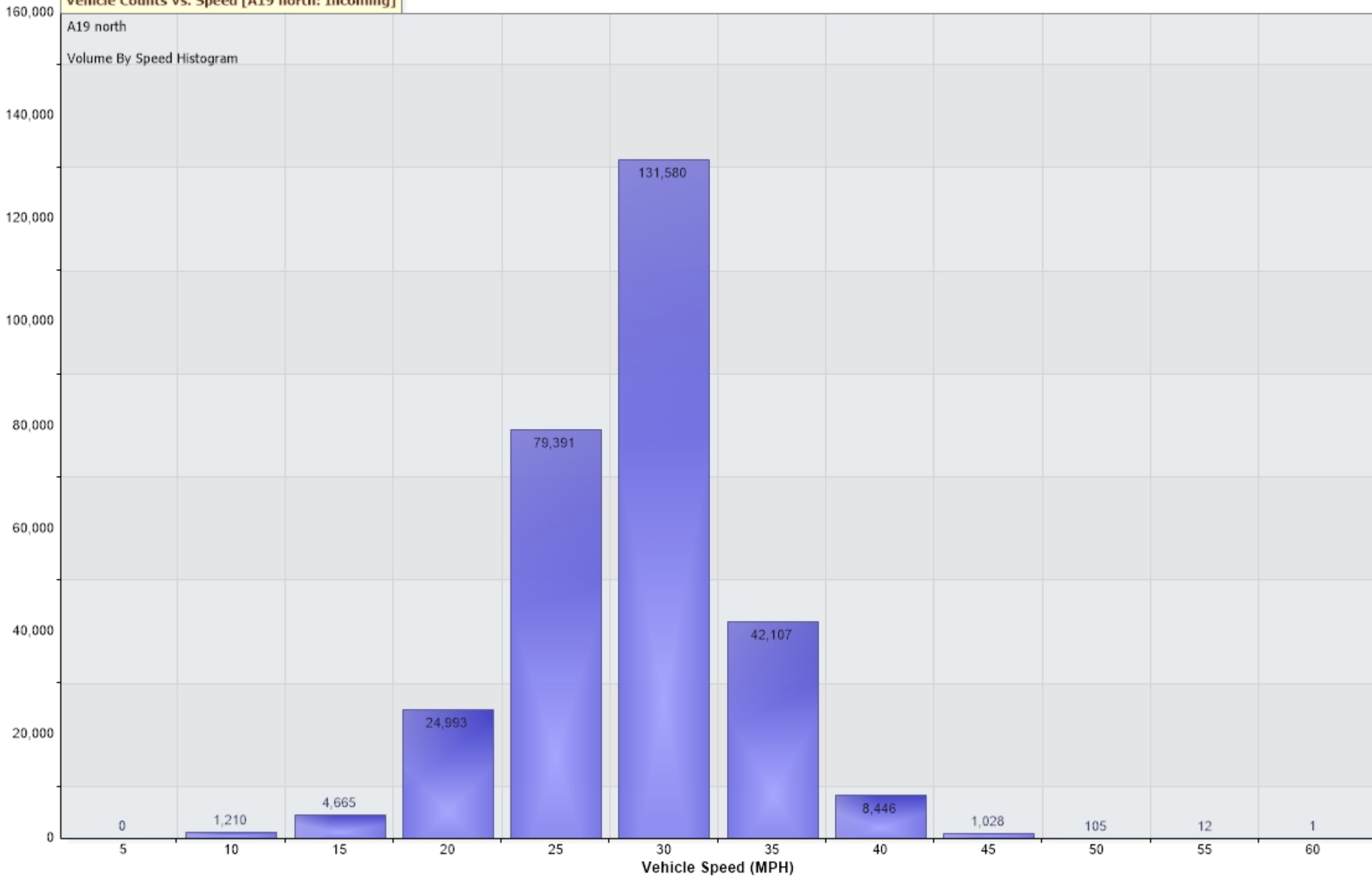
Vehicle Counts Vs. Speed [A19 north: Incoming]
