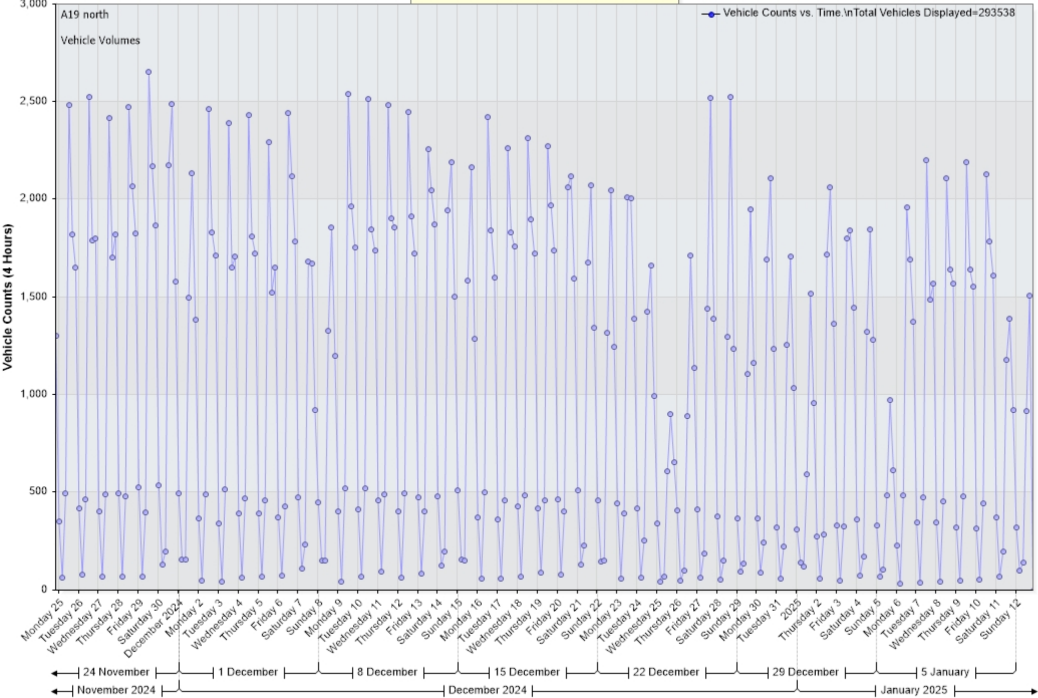
Vehicle Counts vs. Time [A19 north: Incoming]
