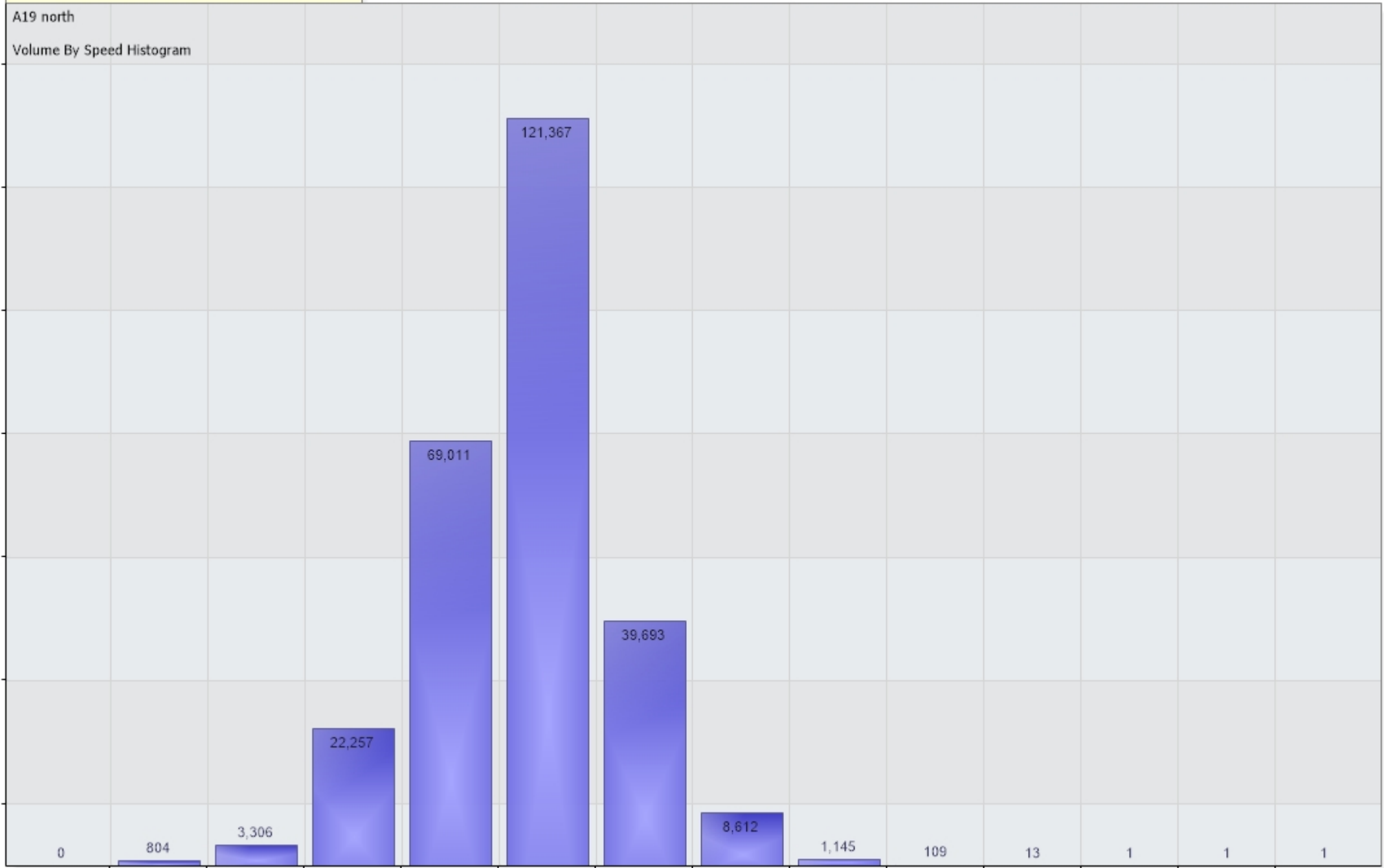
Vehicle Counts Vs. Speed [A19 north: Incoming]
