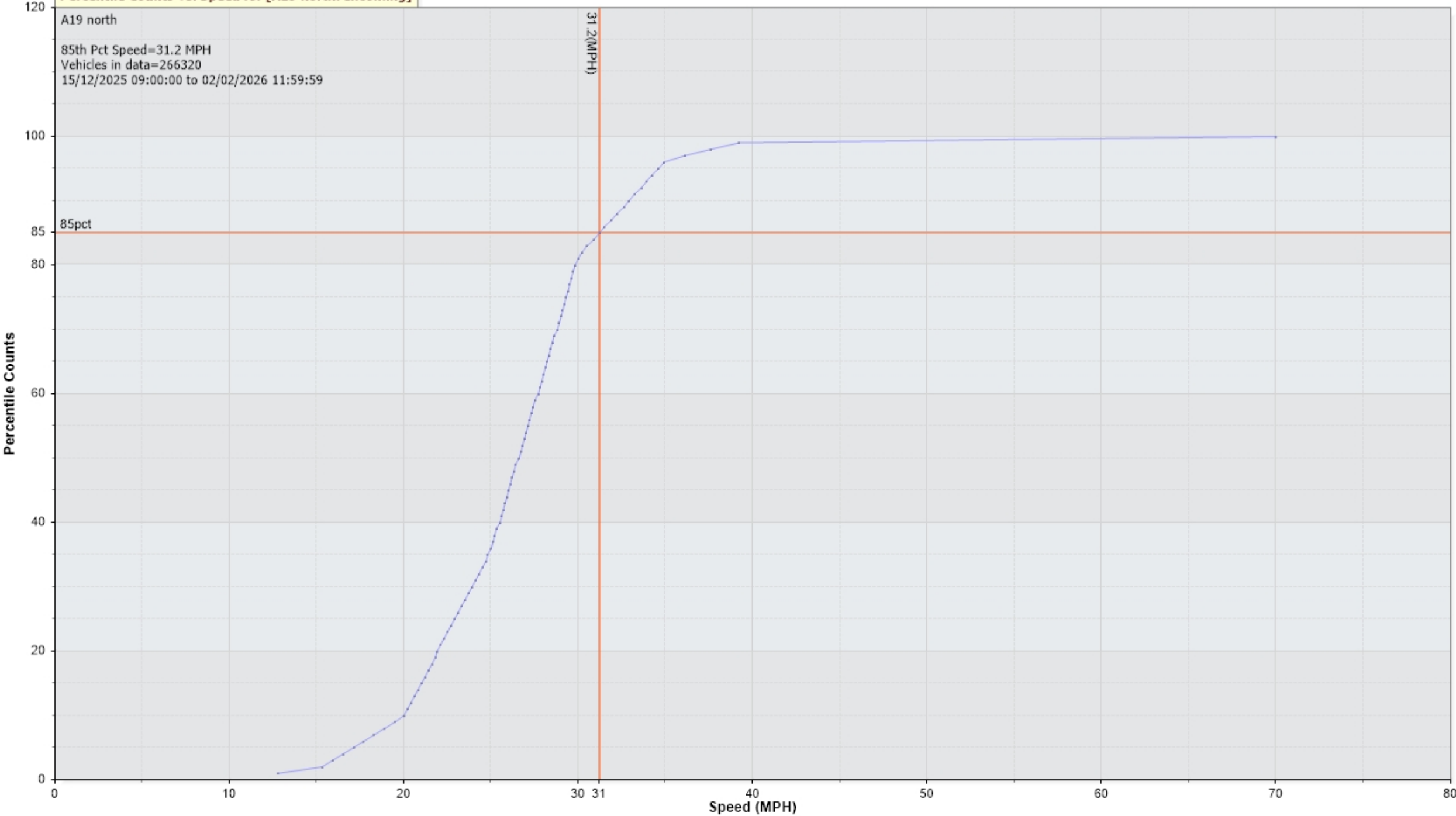
Percentile Counts Vs. Speed for [A19 north: Incoming]
