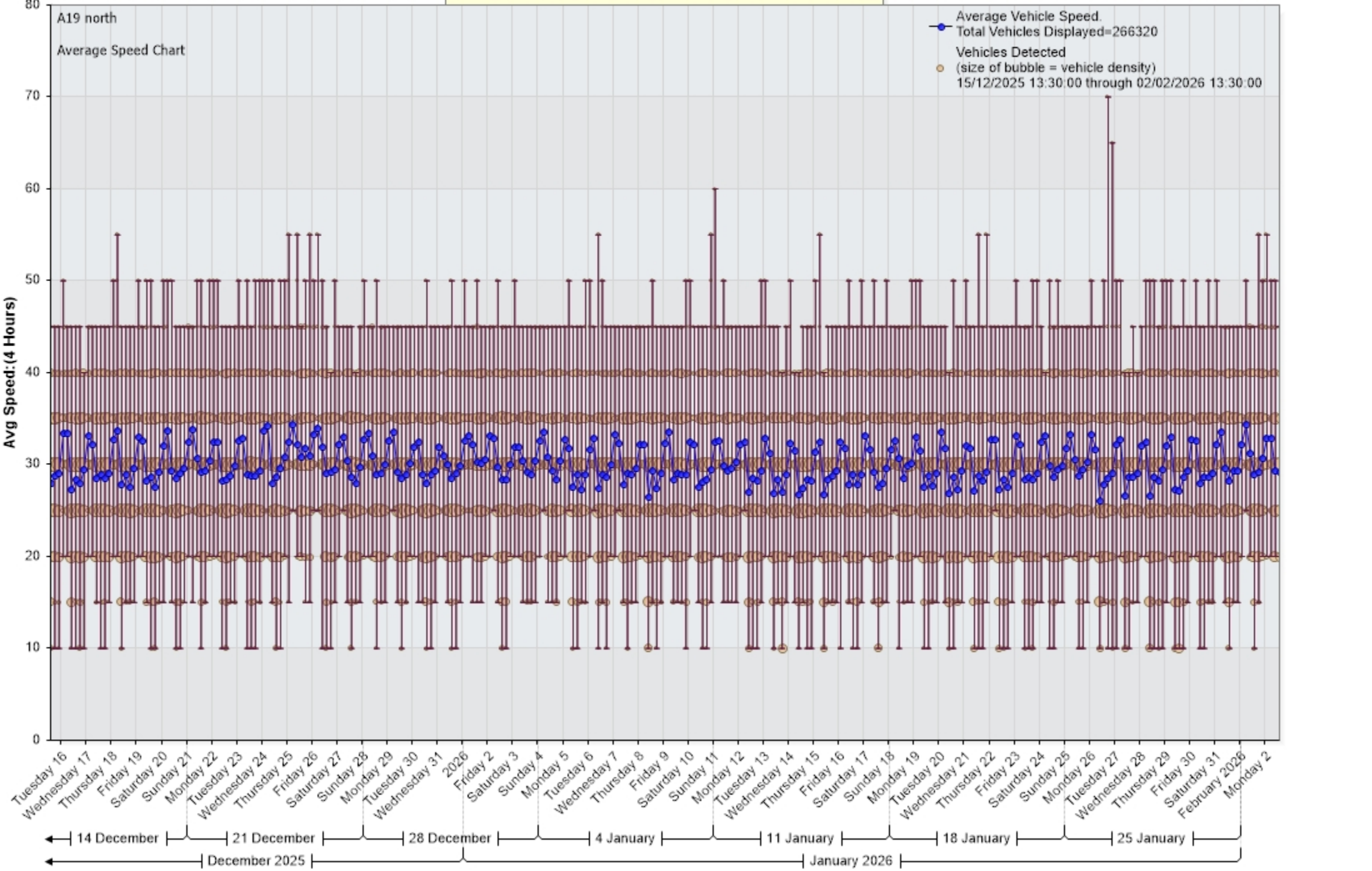
Average Vehicle Speed (MPH) vs. Time [A19 north:Incoming]
