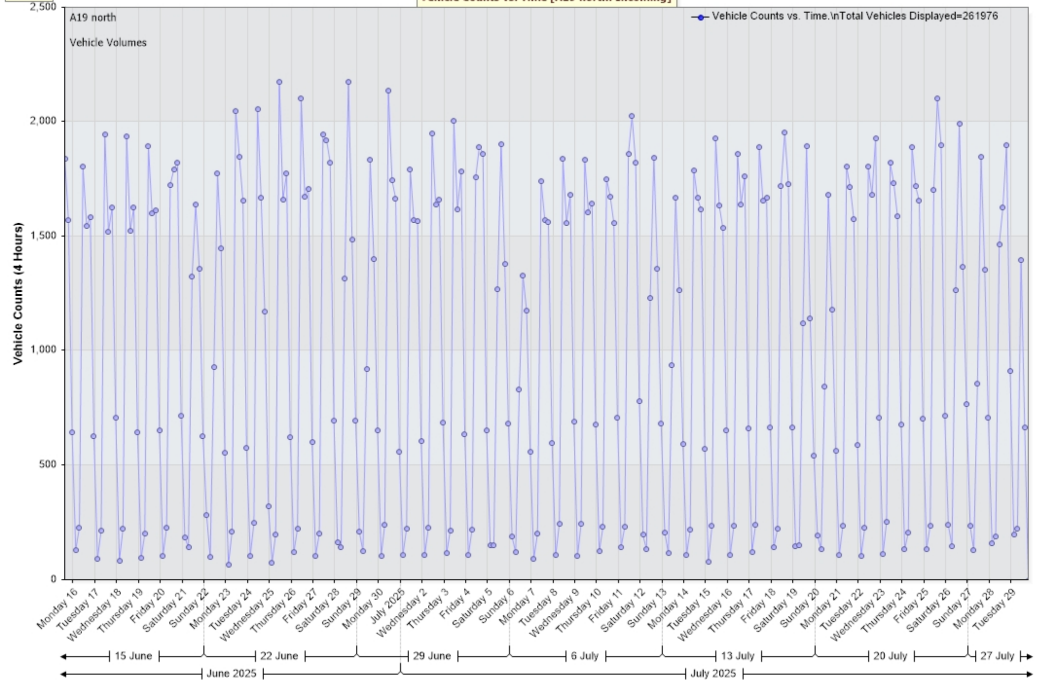
Vehicle Counts vs. Time [A19 north: Incoming]
