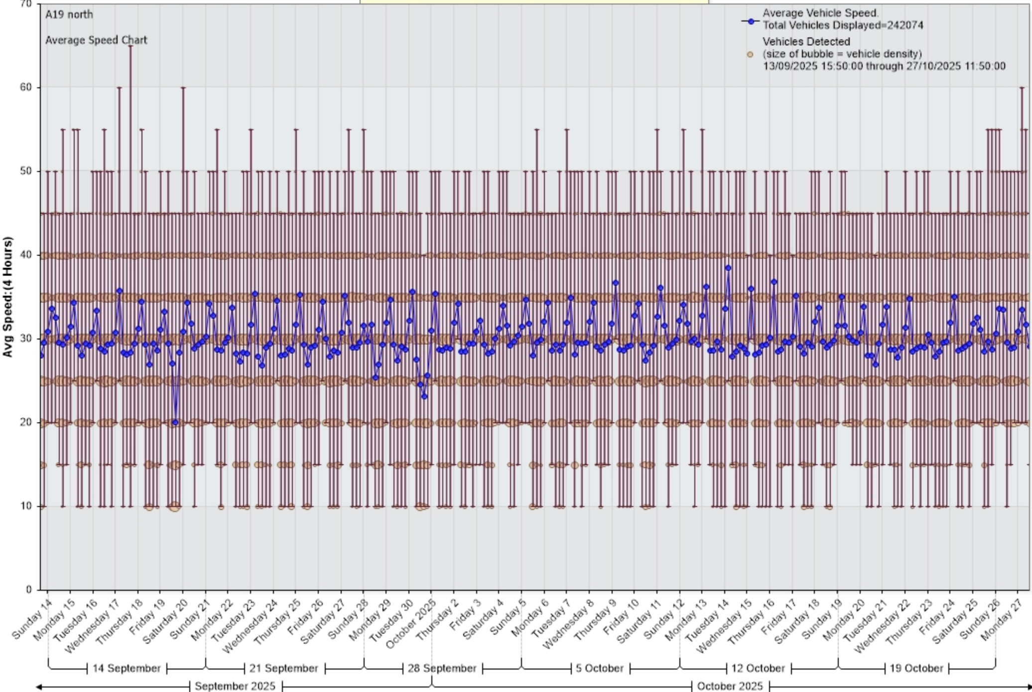
Average Vehicle Speed (MPH) vs. Time [A19 north:Incoming]
