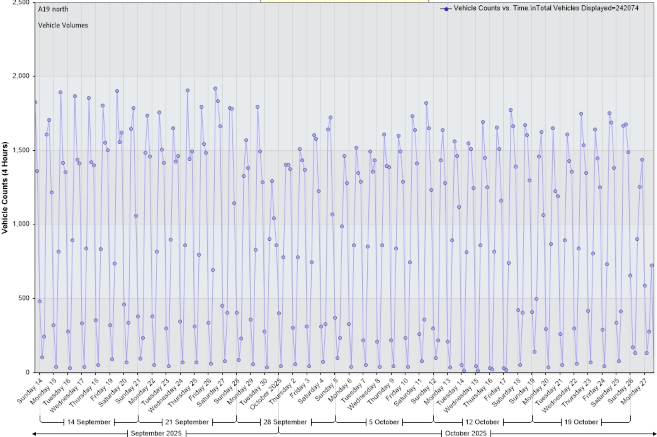
Vehicle Counts vs. Time [A19 north: Incoming]
