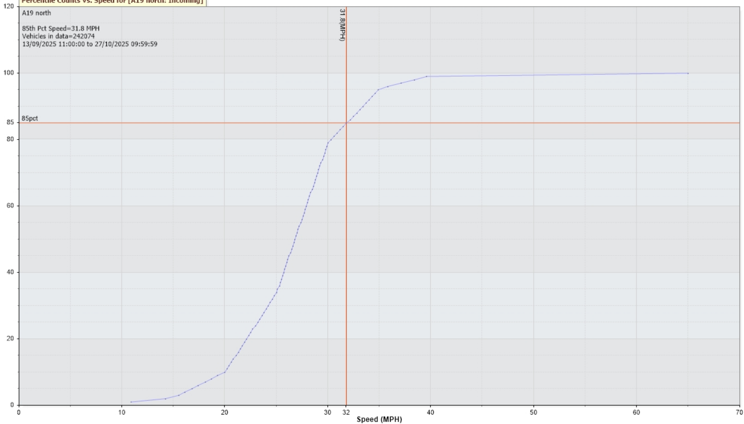
Percentile Counts Vs. Speed for [A19 north: Incoming]
