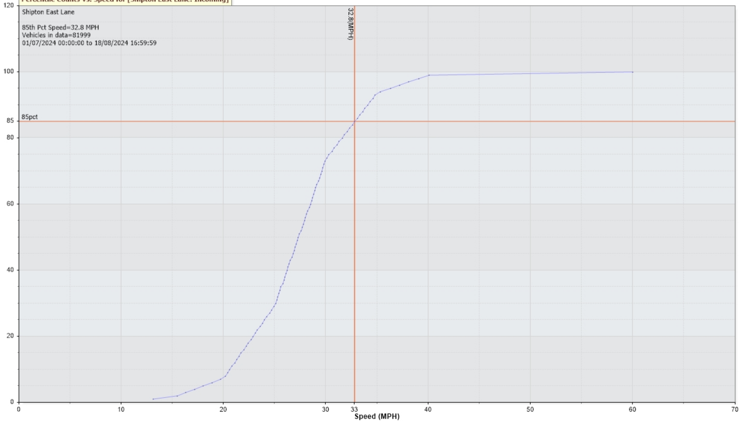
Percentile Counts Vs. Speed for [Shipton East Lane: Incoming]
