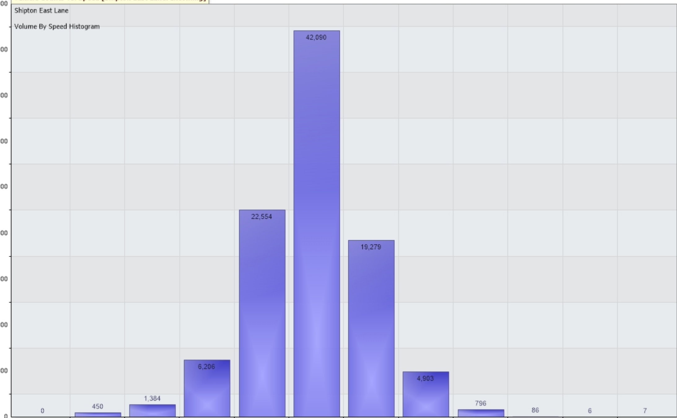
Vehicle Counts Vs. Speed [Shipton East Lane: Incoming]
