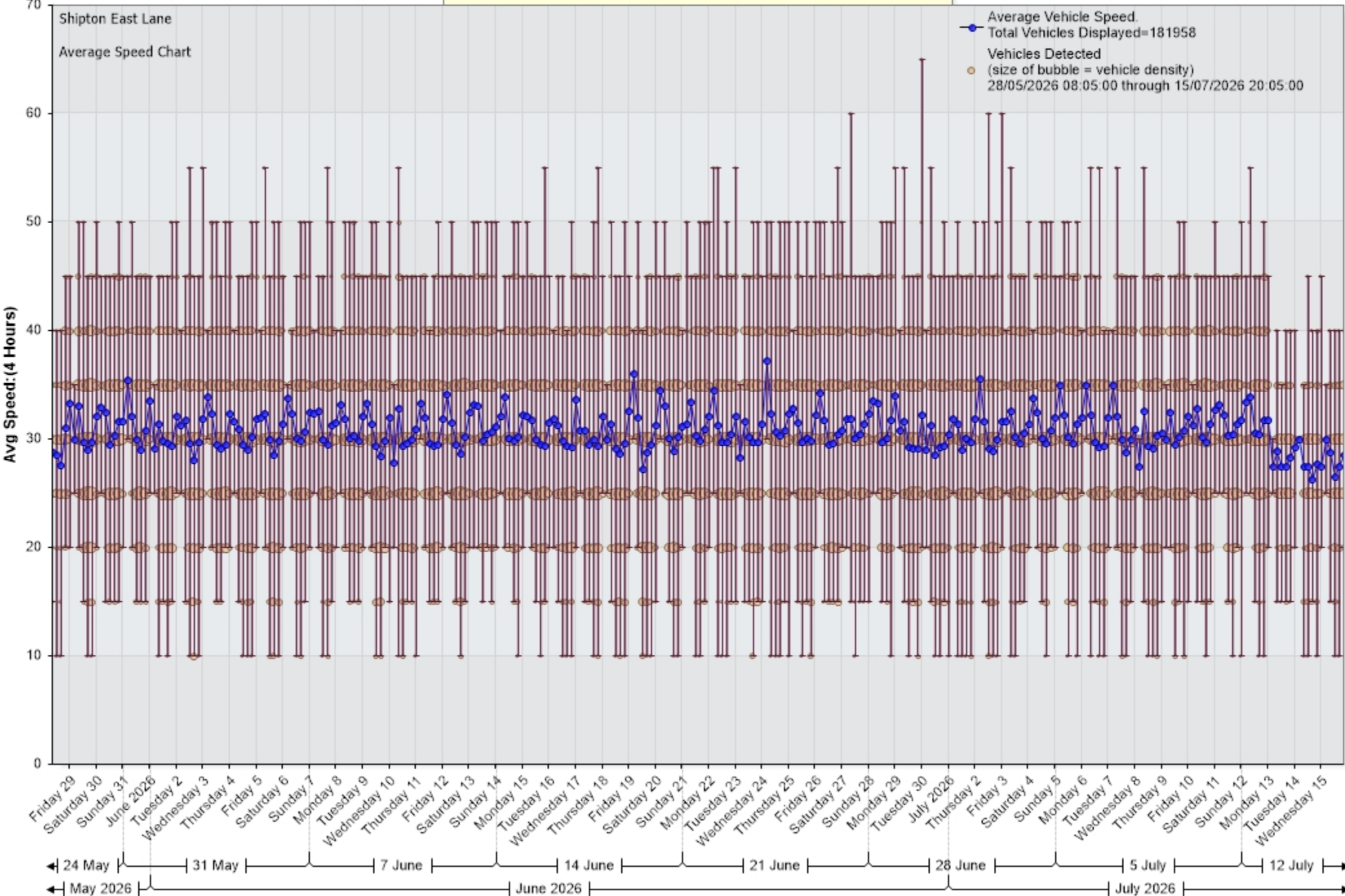
Average Vehicle Speed (MPH) vs. Time [Shipton East Lane:Incoming]
