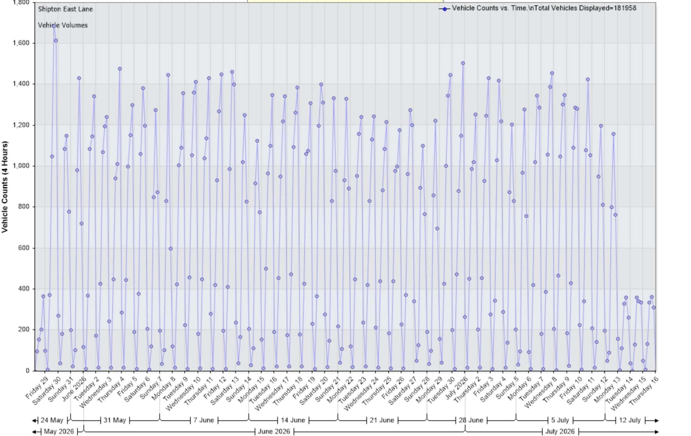
Vehicle Counts vs. Time [Shipton East Lane: Incoming]
