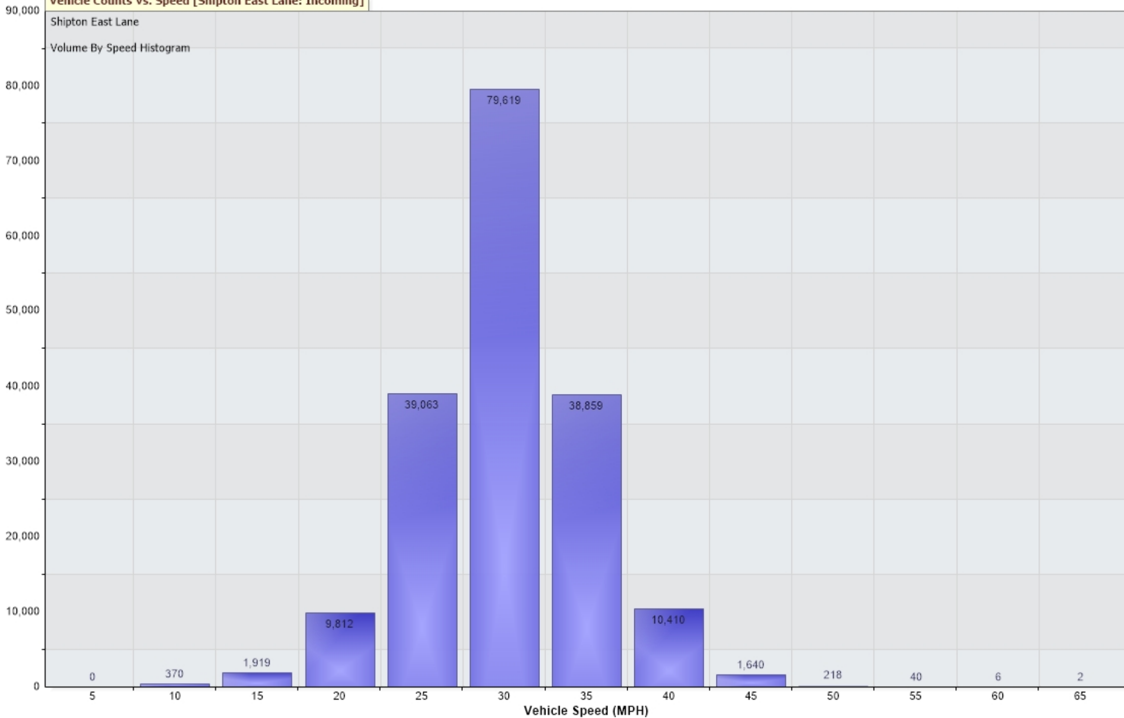
Vehicle Counts Vs. Speed [Shipton East Lane: Incoming]
