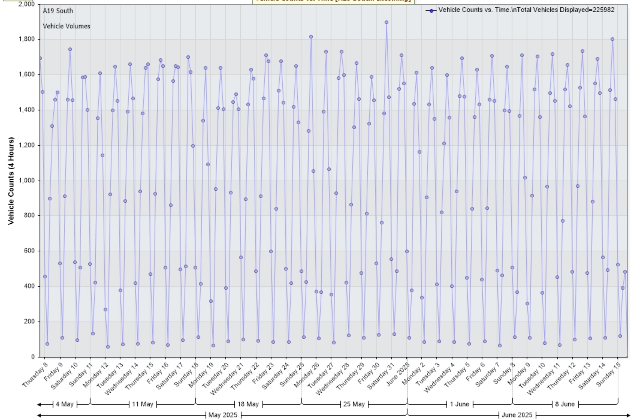
Vehicle Counts vs. Time [A19 South: Incoming]
